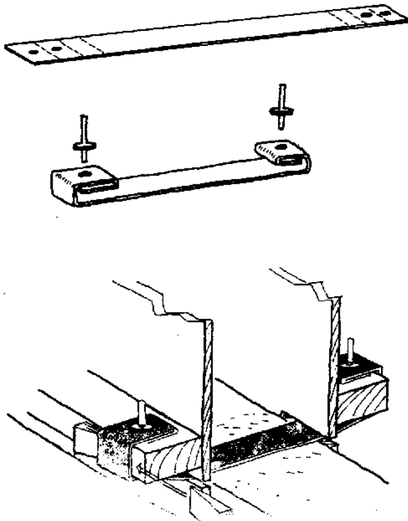
Figure 75. Thin metal strips such as these can be wed instead of bolts to tie rammed earth forms together.
