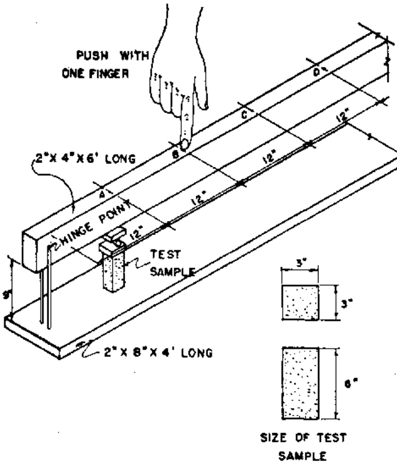
Figure 94. Simple lever tester for soils.
