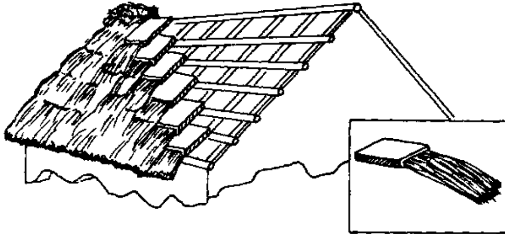
Figure 89. A thatched-earth tile roof of this design proved successful in research studies in India.
