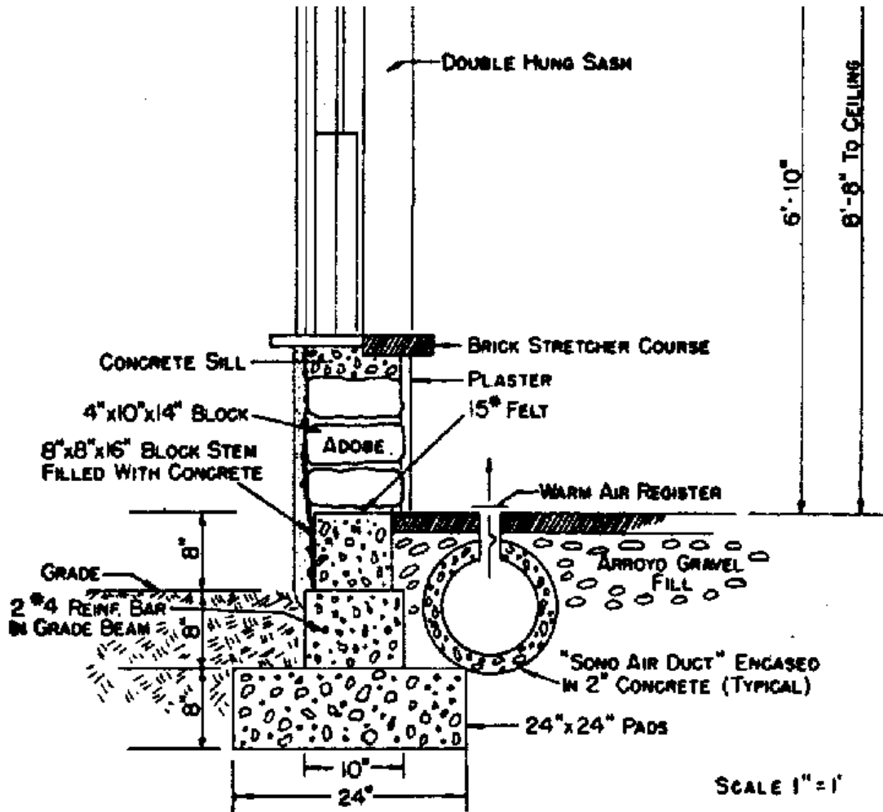
Figure 64. A builder in Albuquerque, N. M., uses this wall section for adobe walls.
