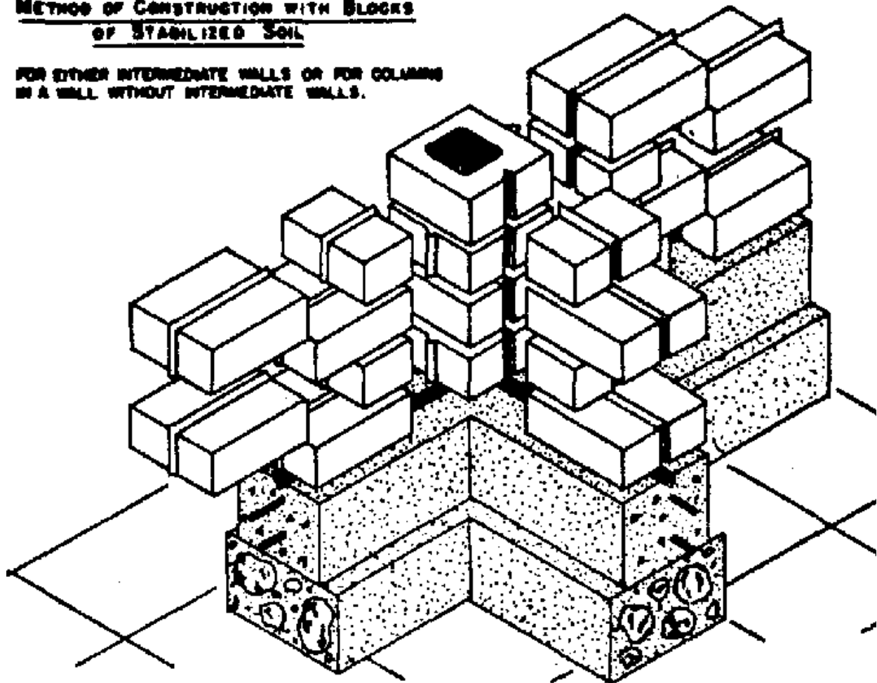
Figure 49. The various shapes of blocks produced by the Land-crete block making machine allow rigid construction of corners and tees.
