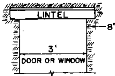
Figure 95. Wood lintel.
