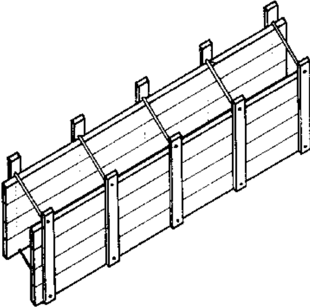
Figure 72. Form for ramming.
