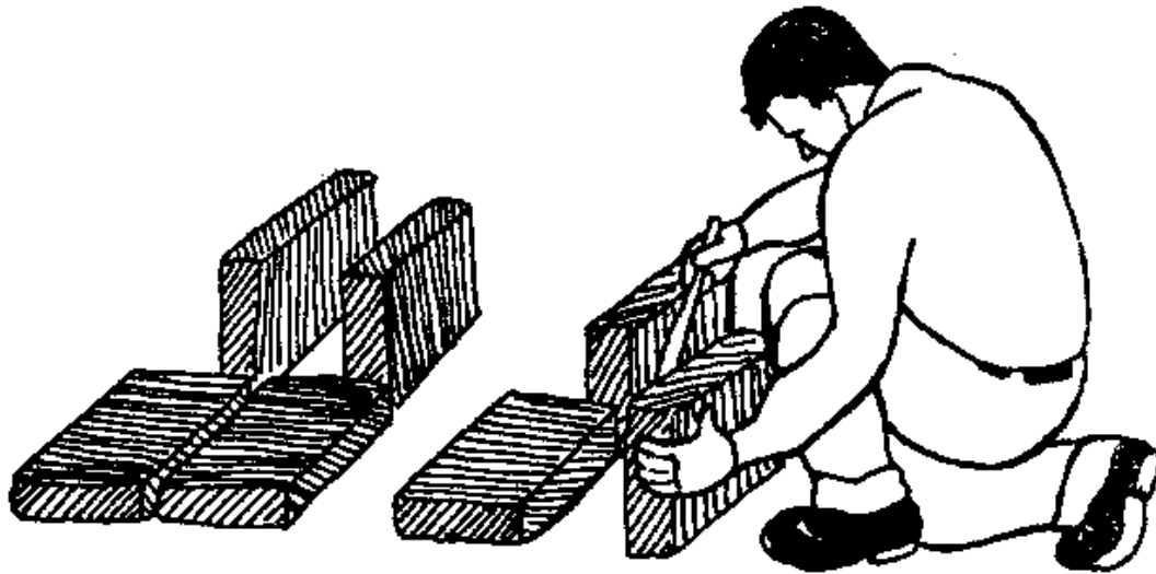
Figure 45. Unstabilized block is turned on edge to dry after two to four days.
